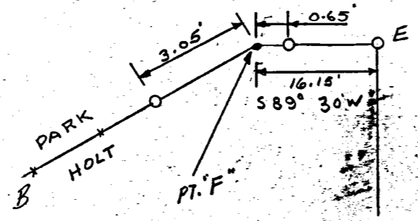
DETAIL PT. "F"
